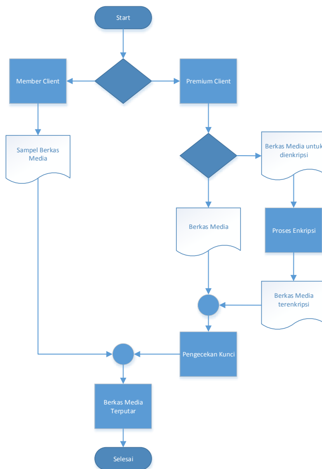
Gambar 1 Flowchart Sistem
