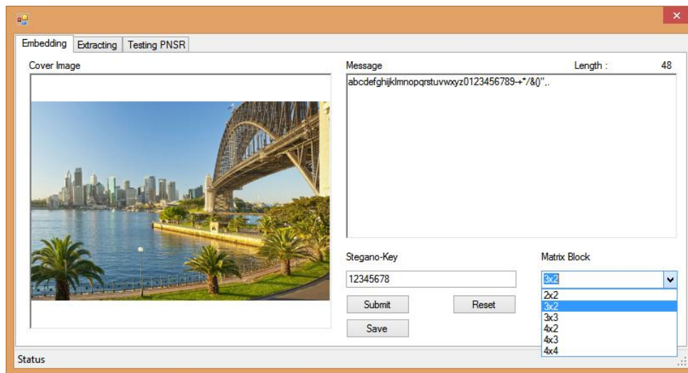
Gambar 6. Form Embedding
