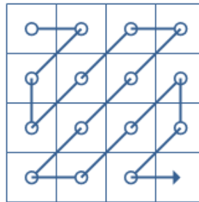
Gambar 4 Zigzag scanning
