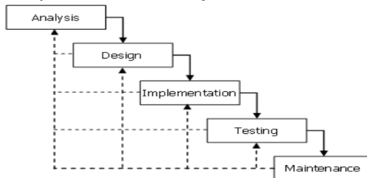
Gambar 1 Metode Waterfall
